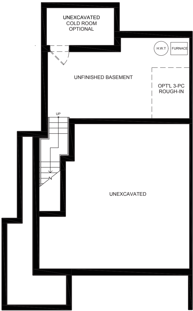
BASEMENT
