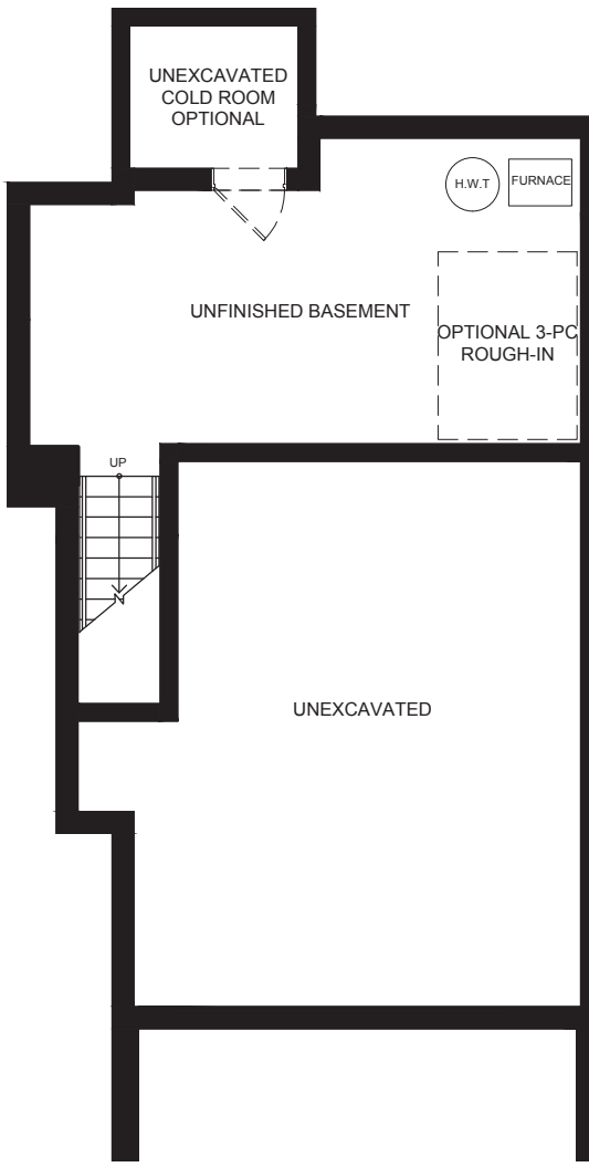
BASEMENT
