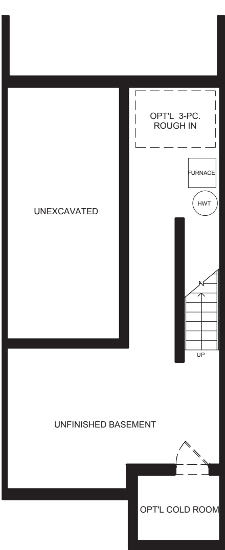
BASEMENT FLOOR
