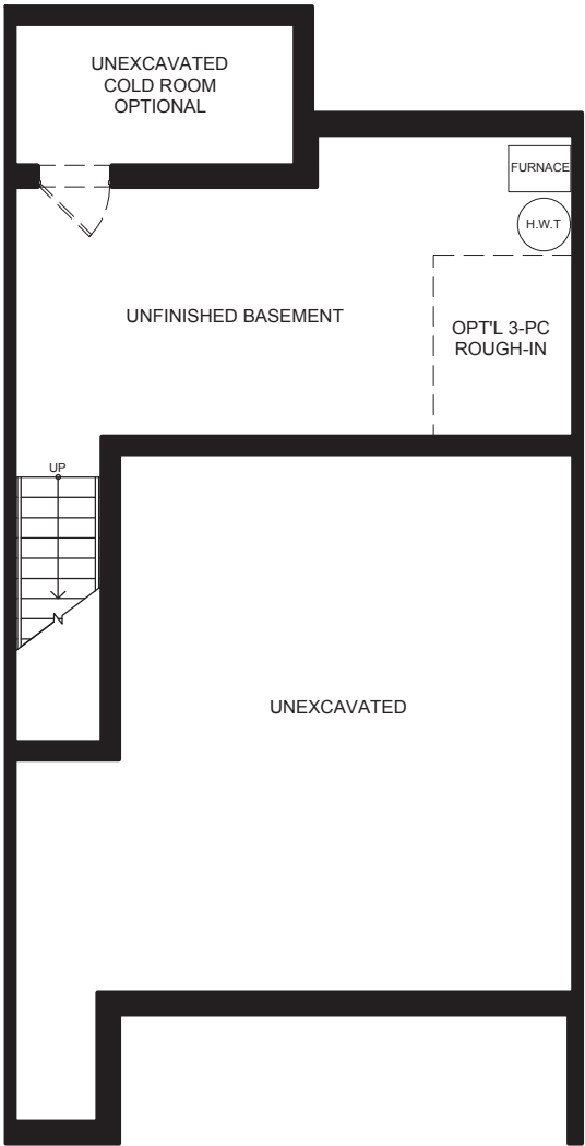
BASEMENT
