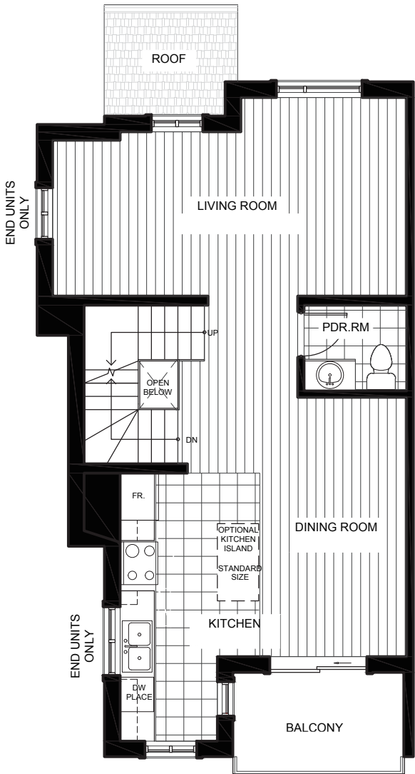
FIRST FLOOR
